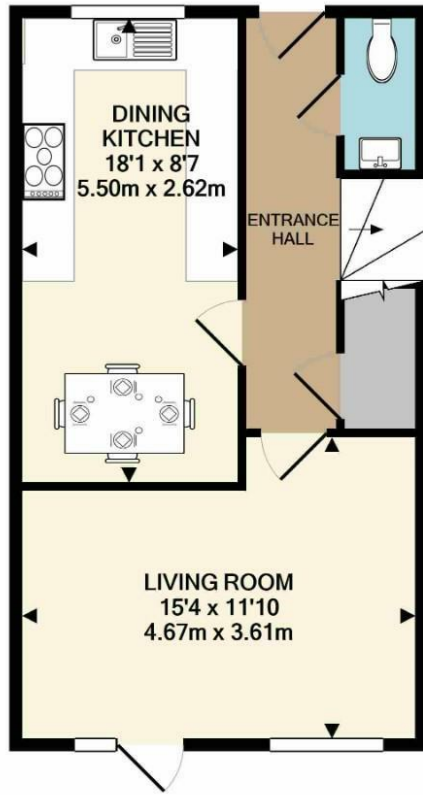
GROUND FLOOR APPROX. FLOOR AREA 430 SQ.FT. (39.9 SQ.M.)
