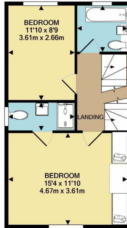
1ST FLOOR APPROX. FLOOR AREA 430 SQ.FT. (39.9 SQ.M.)
